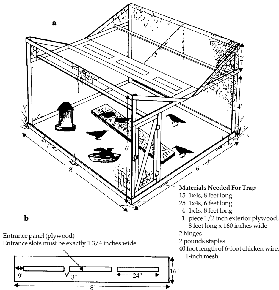
Fig. 11. Starling decoy trap: (a) assembled view and (b) details of the entrance panel. Side and end panels are covered with wire on the outside; top panels are covered on the inside of the frame.
