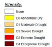
September 29, 2020 Drought Monitor
