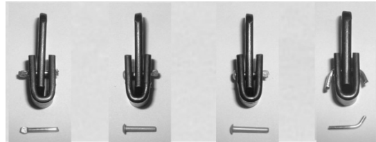
250-lb 285-lb 320-lb 250-lb Neck-Snare Neck-Snare Neck-Snare Foot-Snare Lock with Lock with Lock with Lock with Aluminum Gold Pin Green Pin Aluminum Pin Pin
